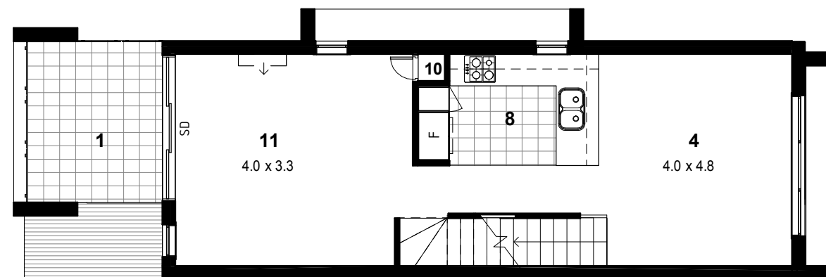
FIRST FLOOR
