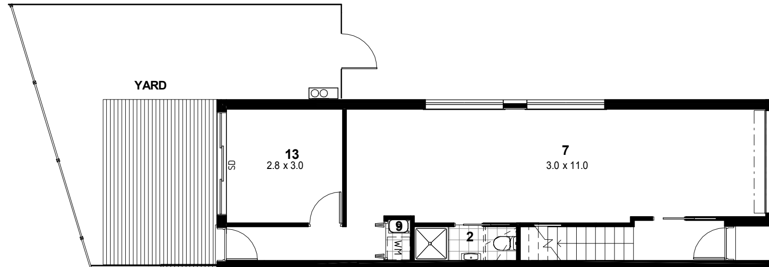
GROUND FLOOR
