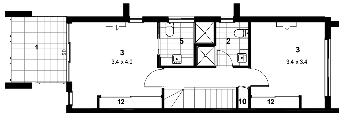
SECOND FLOOR
