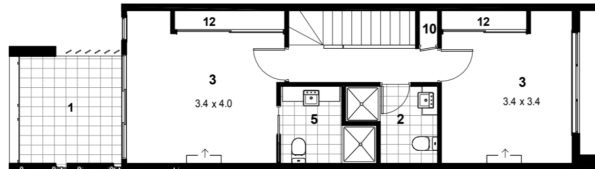
SECOND FLOOR
