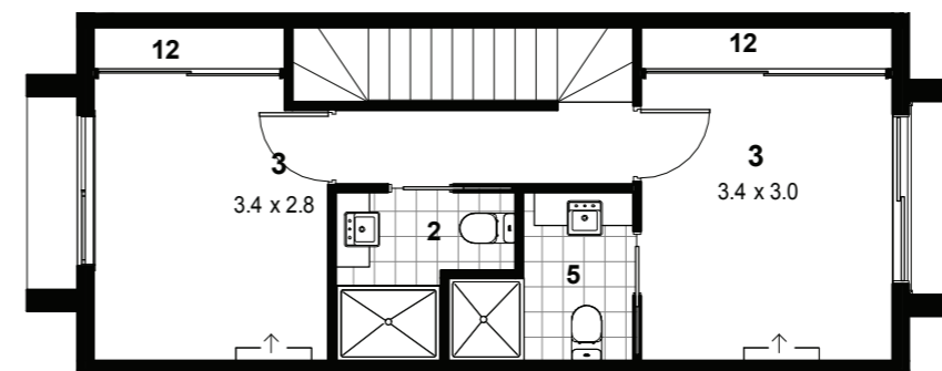
SECOND FLOOR
