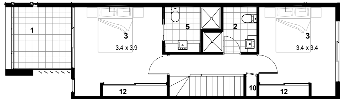
SECOND FLOOR
